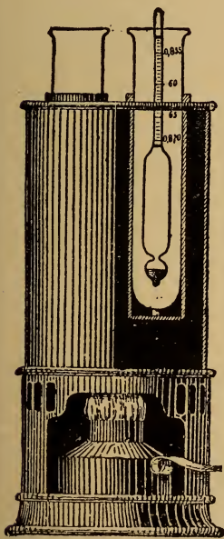
Fig. 56. KOENIG'S APPARATUS FOR DISTINGUISHING MARGARINE FROM BUTTER.
